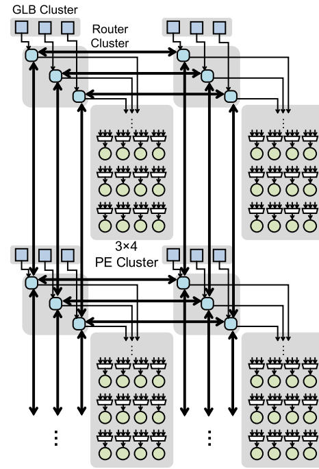
Fig. 10. Hierarchical mesh network for input activations. This only shows the top 2 \times 2 of the entire 8 \times 2 cluster array.
