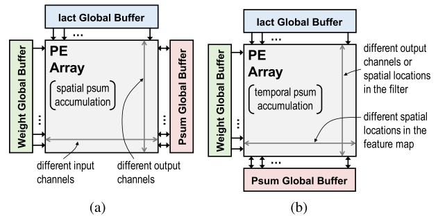
Fig. 3. Two common DNN accelerator designs: (a) Spatial accumulation array [29]–[32]: iacts are reused vertically and psums are accumulated horizontally. (b) Temporal accumulation array [15]–[17]: iacts are reused vertically and weights are reused horizontally.
